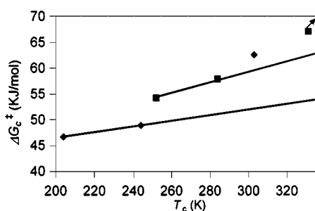
Figure 3. Linear plot of \Delta G_c^\ddagger (kJ/mol) versus T_c (K) for complex 4 ( 1.41 \times 10^{-2} M; see Table 3): CDCl_3 (squares); [D_6] acetone (diamonds); allylic interchange (—)
