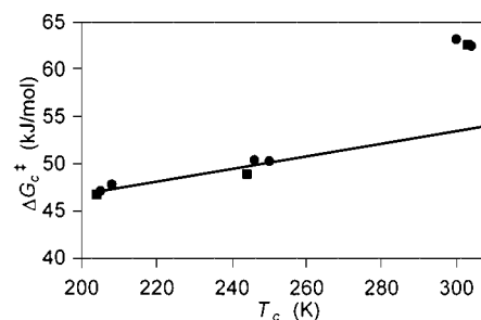
Figure 2. Linear plot of \Delta G_c^\ddagger (kJ/mol) versus T_c (K) for complexes 4 and 6 in [D_6] acetone ( 1.41 \times 10^{-2} M; see Table 3): 4 (squares); 6 (circles); allylic interchange (—); R^2 = 0.9706
