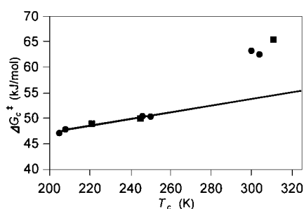
Figure 4. Linear plot of \Delta G_c^\ddagger (kJ/mol) versus T_c (K) for complex 6 ( 1.41 \times 10^{-2} M; see Table 3): CD_2Cl_2 (squares); [D_6] acetone (circles); allylic interchange (—); R^2 = 0.9914
