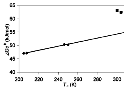
Figure 1. Linear plot of \Delta G_c^\ddagger (kJ/mol) versus T_c (K) for complex 6 in [D_6] acetone ( 1.41 \times 10^{-2} M) using data from 300 and 500 MHz NMR spectrometers (see Table 3): allylic interchange (diamonds, —); ( R^2 = 0.9985 ); H^4-H^6 interchange (squares)
